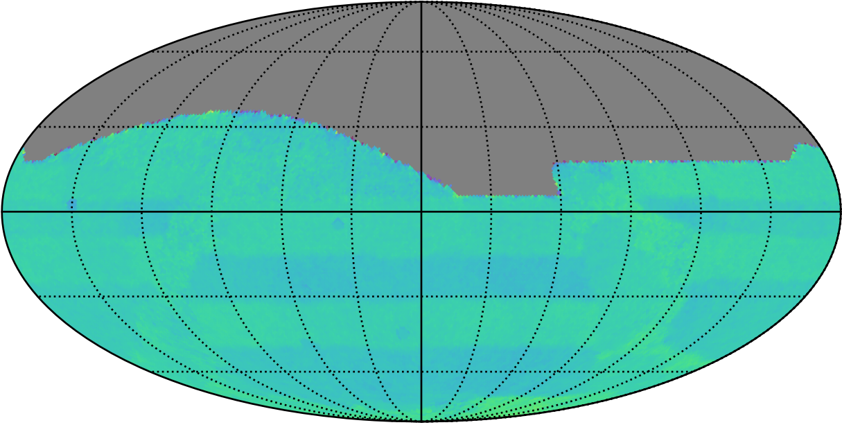
ddf_acor_sf10_lsf40_lsr50_v3.4_10yrs All sky: Normalized Proper Motion Uncert @ 20.5
