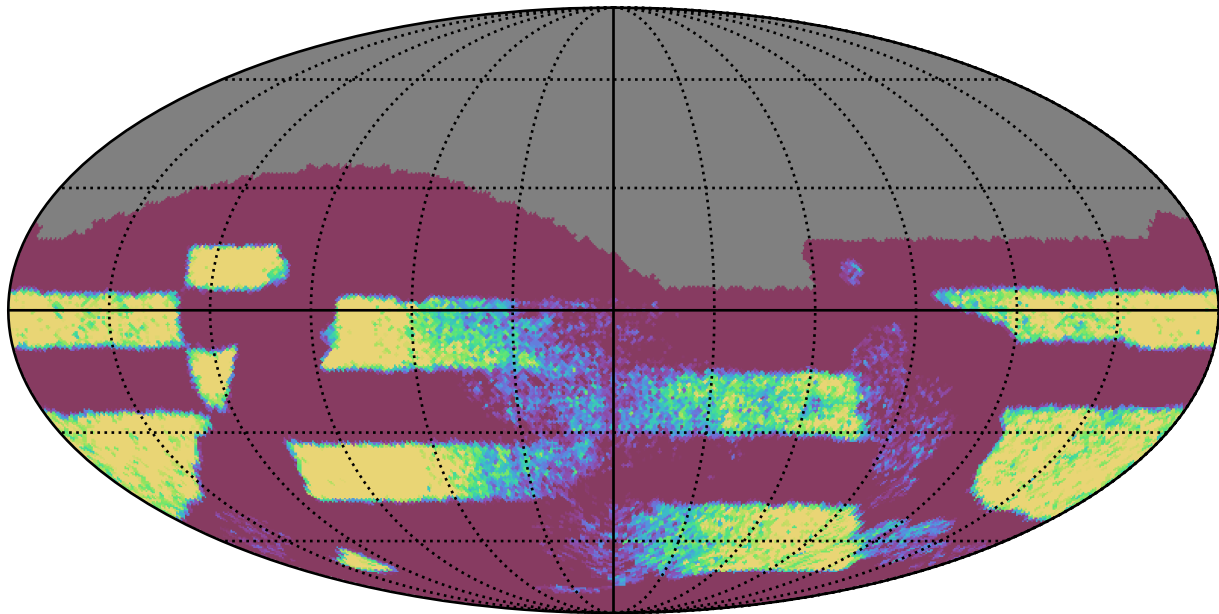
ddf_acor_sf10_lsf40_lsr50_v3.4_10yrs Yr 3-4 all bands: NVisits
