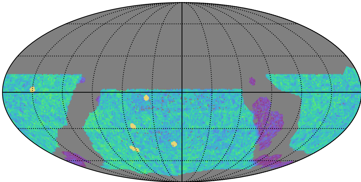
ddf_acor_sf10_lsf40_lsr50_v3.4_10yrs WFD u band: NVisits
