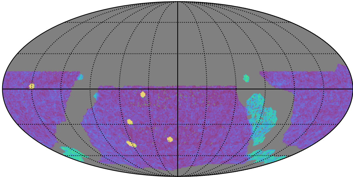
ddf_acor_sf10_lsf40_lsr50_v3.4_10yrs WFD g band: NVisits
