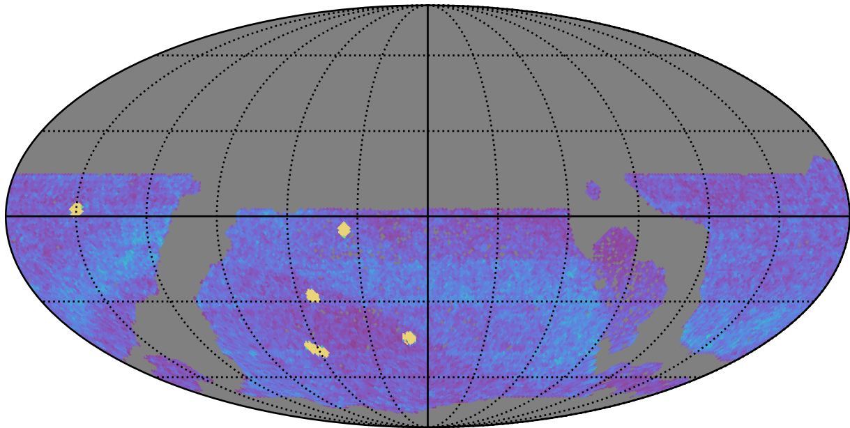
ddf_acor_sf10_lsf40_lsr50_v3.4_10yrs WFD all bands: NVisits
