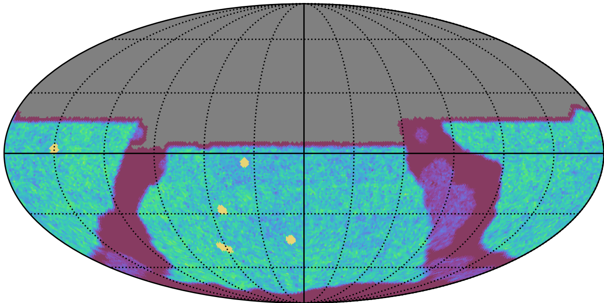
ddf_acor_sf10_lsf40_lsr50_v3.4_10yrs All sky u band: NVisits
