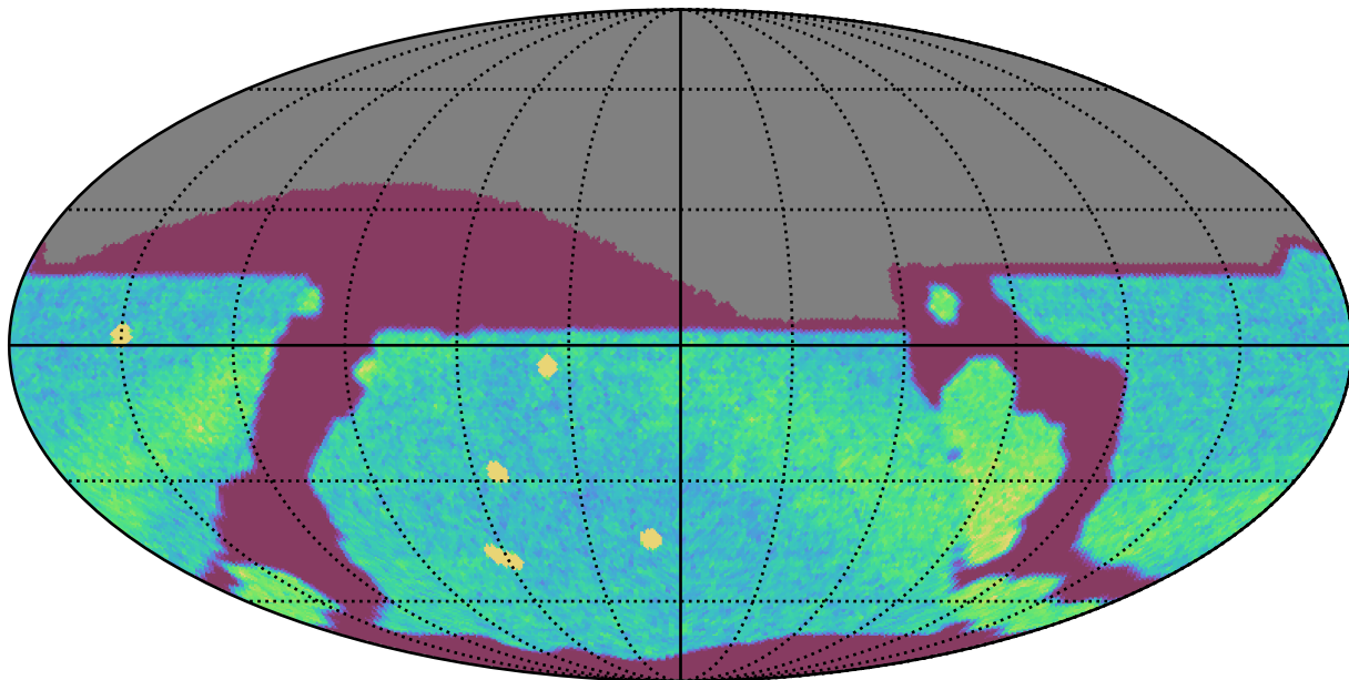
ddf_acor_sf10_lsf40_lsr50_v3.4_10yrs All sky r band: NVisits
