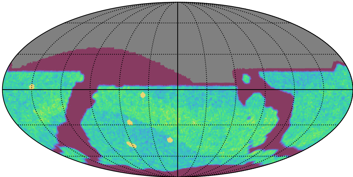
ddf_acor_sf10_lsf40_lsr50_v3.4_10yrs All sky i band: NVisits
