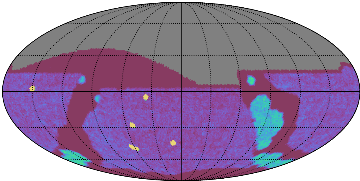
ddf_acor_sf10_lsf40_lsr50_v3.4_10yrs All sky g band: NVisits
