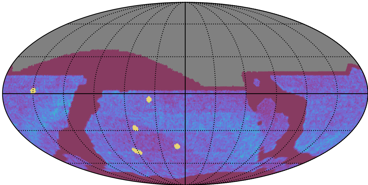
ddf_acor_sf10_lsf40_lsr50_v3.4_10yrs All sky all bands: NVisits
