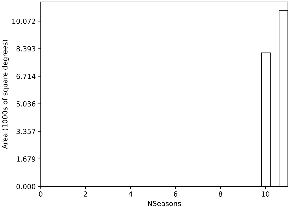
ddf_acor_sf10_lsf40_lsr50_v3.4_10yrs WFD all bands: NSeasons
