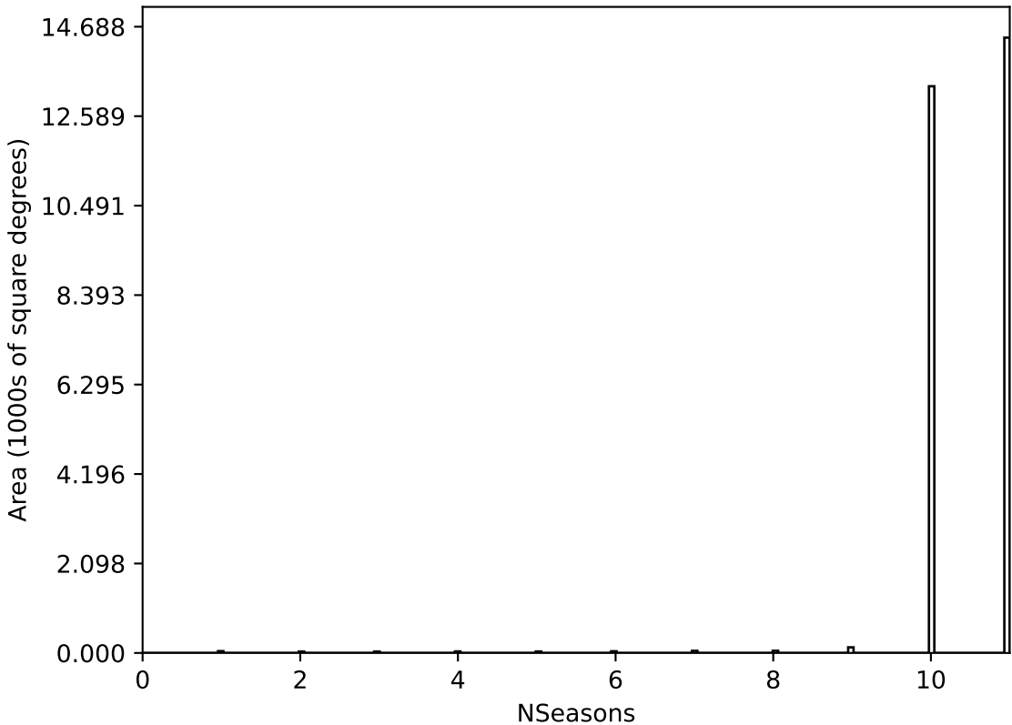
ddf_acor_sf10_lsf40_lsr50_v3.4_10yrs All sky all bands: NSeasons
