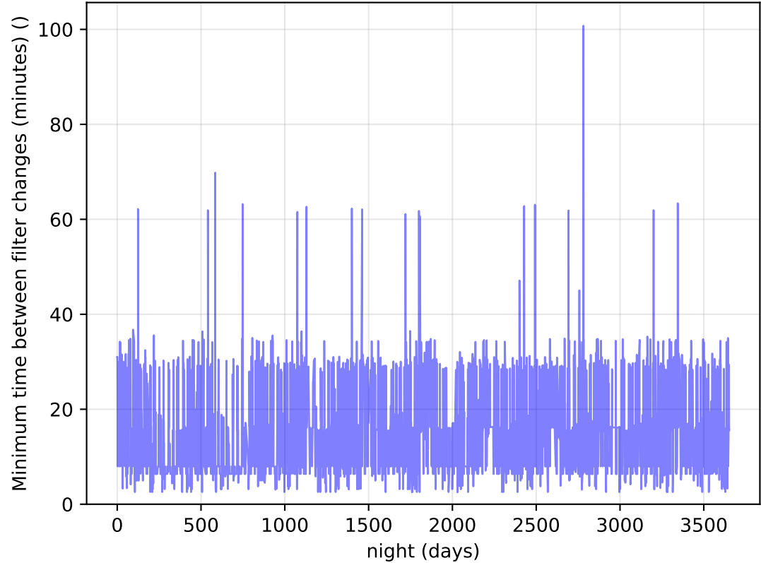
ddf_acor_sf10_Isf40_Isr50_v3.4_10yrs Per Night: Minimum time between filter changes (minutes)
