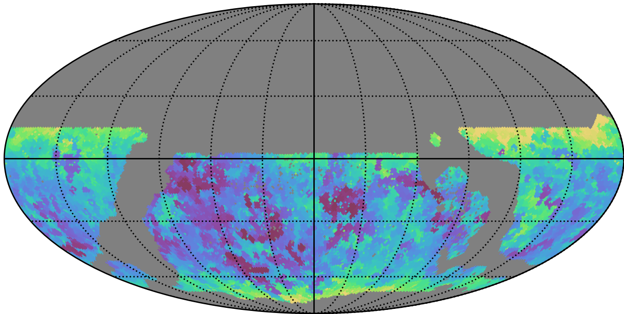
ddf_acor_sf10_lsf40_lsr50_v3.4_10yrs WFD z band: Min seeingEff
