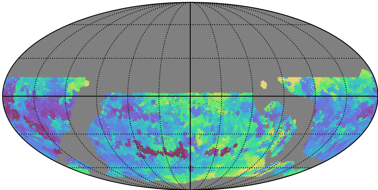
ddf_acor_sf10_lsf40_lsr50_v3.4_10yrs WFD u band: Min seeingEff
