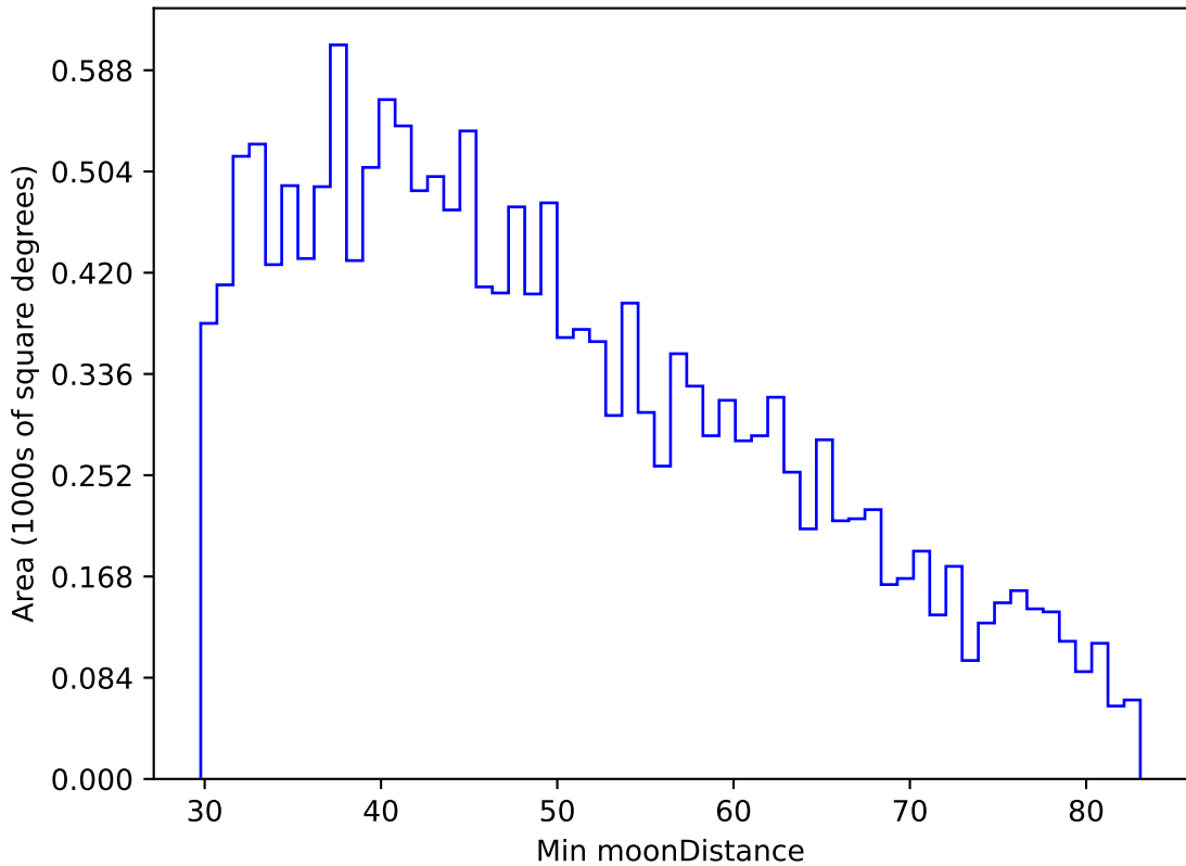
ddf_acor_sf10_lsf40_lsr50_v3.4_10yrs WFD u band: Min moonDistance
