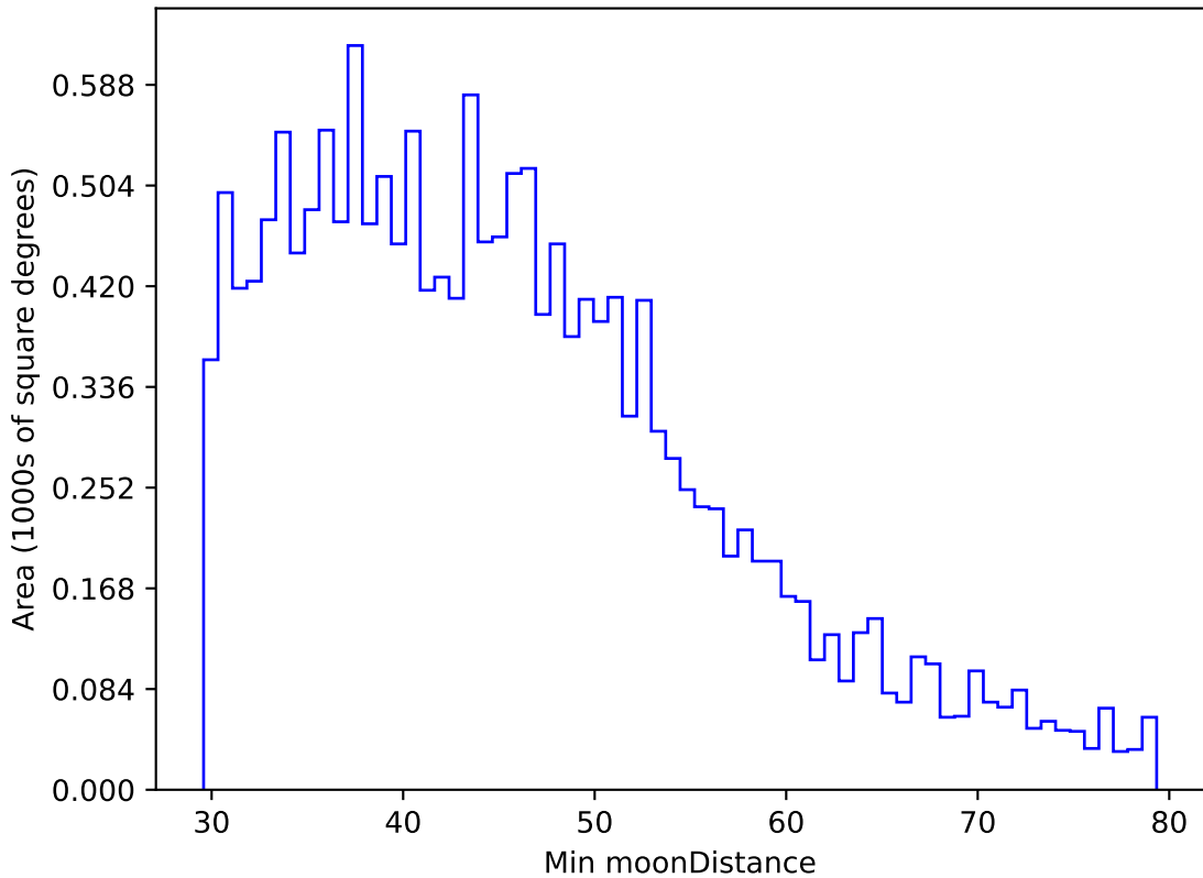
ddf_acor_sf10_lsf40_lsr50_v3.4_10yrs WFD g band: Min moonDistance
