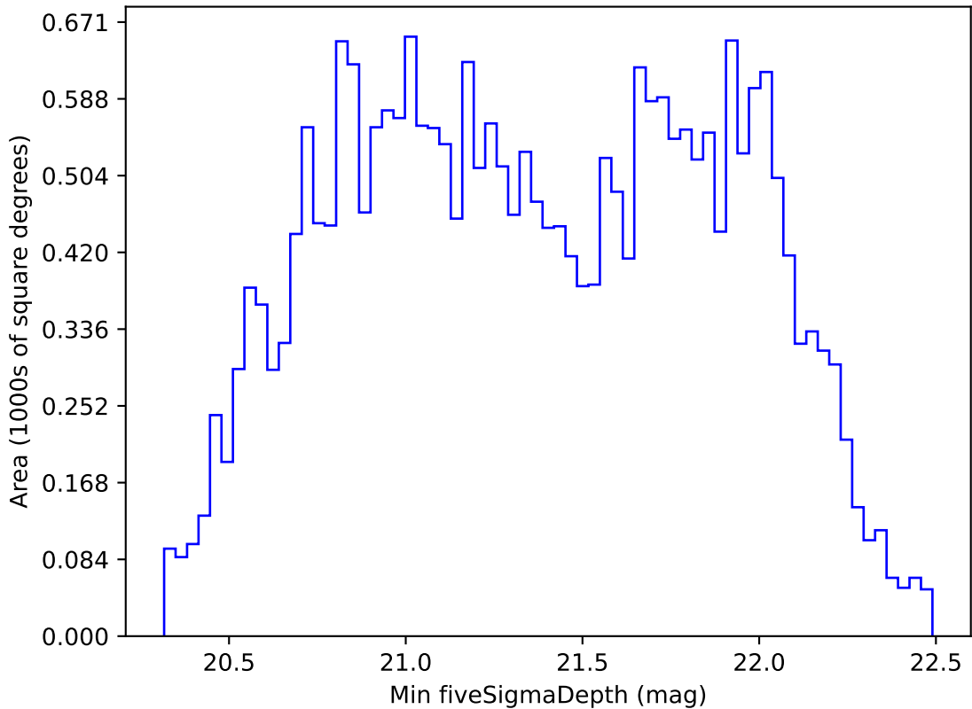
ddf_acor_sf10_lsf40_lsr50_v3.4_10yrs All sky z band: Min fiveSigmaDepth
