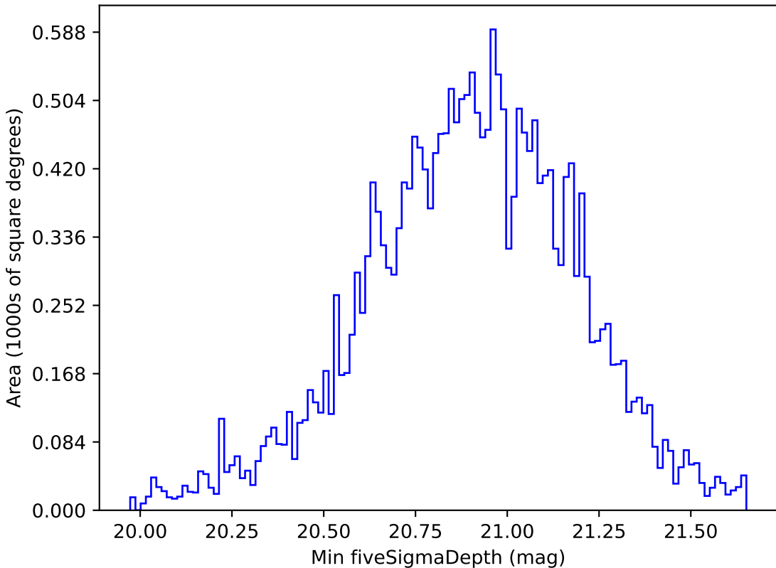
ddf_acor_sf10_lsf40_lsr50_v3.4_10yrs All sky y band: Min fiveSigmaDepth
