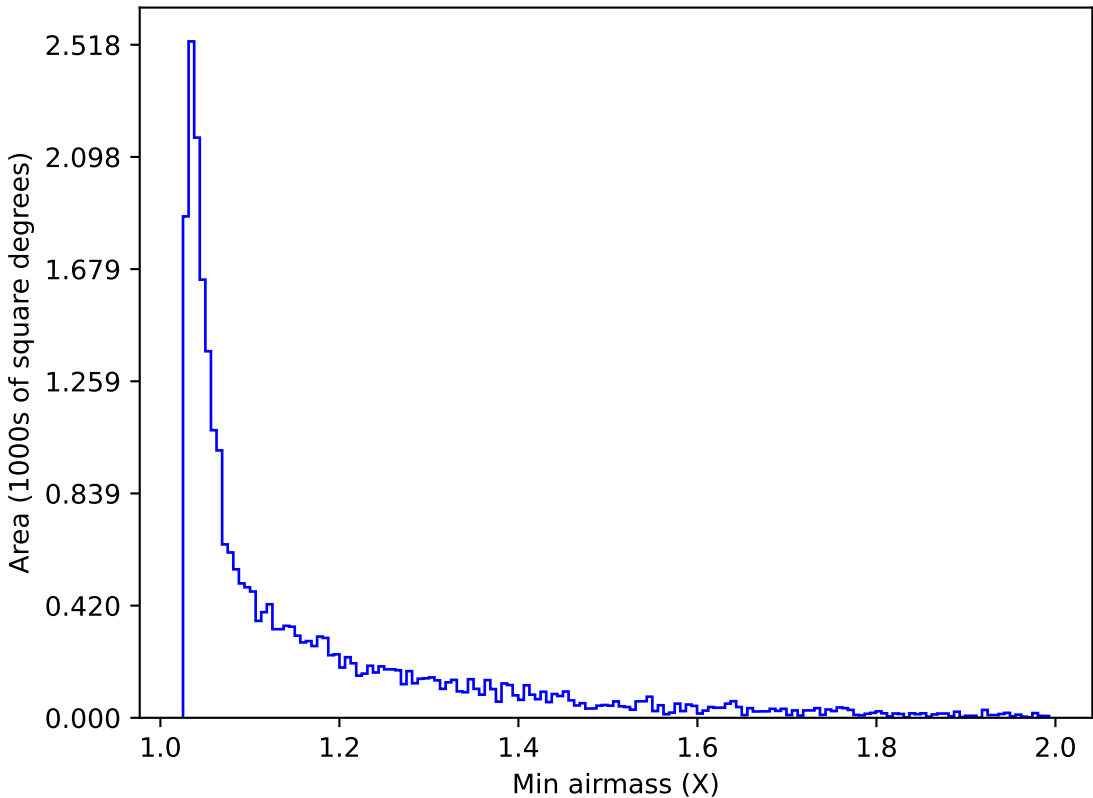
ddf_acor_sf10_lsf40_lsr50_v3.4_10yrs Yr 1 z band: Min airmass
