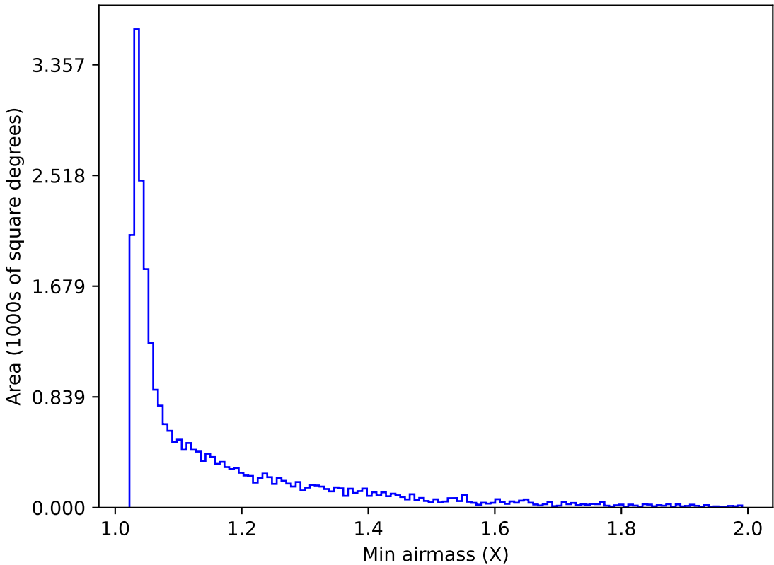
ddf_acor_sf10_lsf40_lsr50_v3.4_10yrs Yr 1 i band: Min airmass
