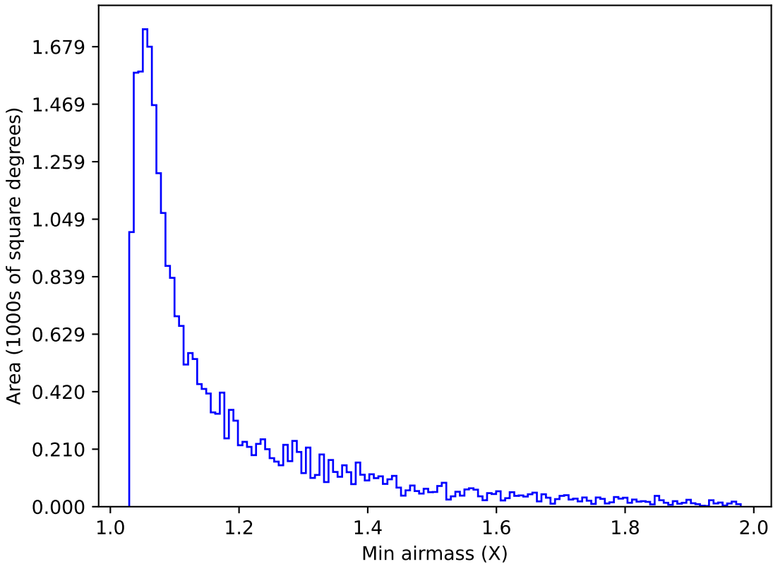
ddf_acor_sf10_lsf40_lsr50_v3.4_10yrs Yr 1 g band: Min airmass
