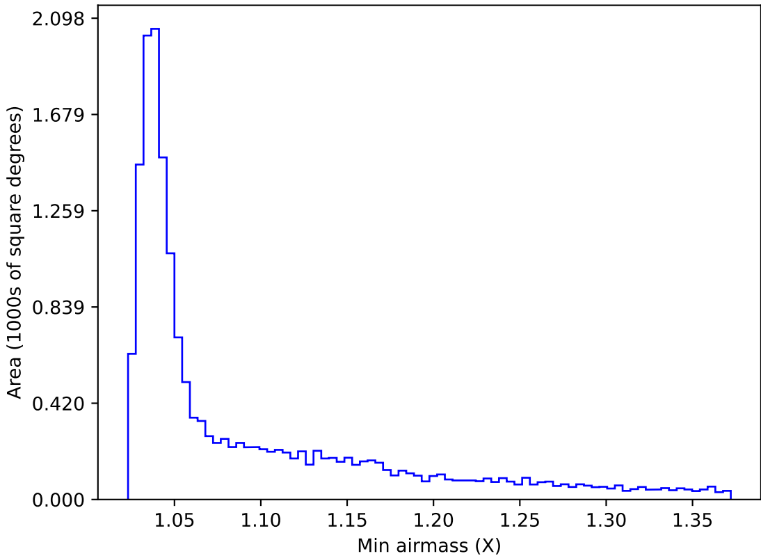
ddf_acor_sf10_lsf40_lsr50_v3.4_10yrs WFD u band: Min airmass
