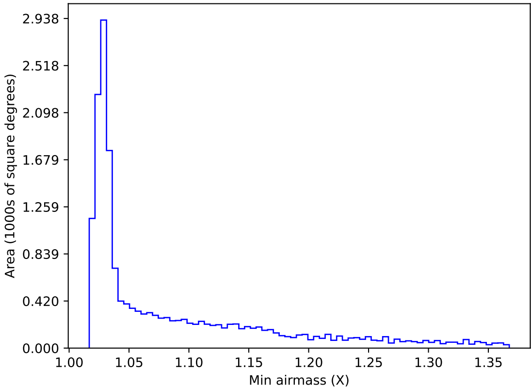
ddf_acor_sf10_lsf40_lsr50_v3.4_10yrs WFD r band: Min airmass
