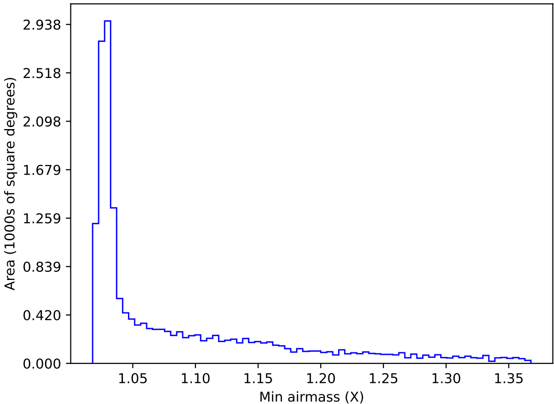
ddf_acor_sf10_lsf40_lsr50_v3.4_10yrs WFD i band: Min airmass
