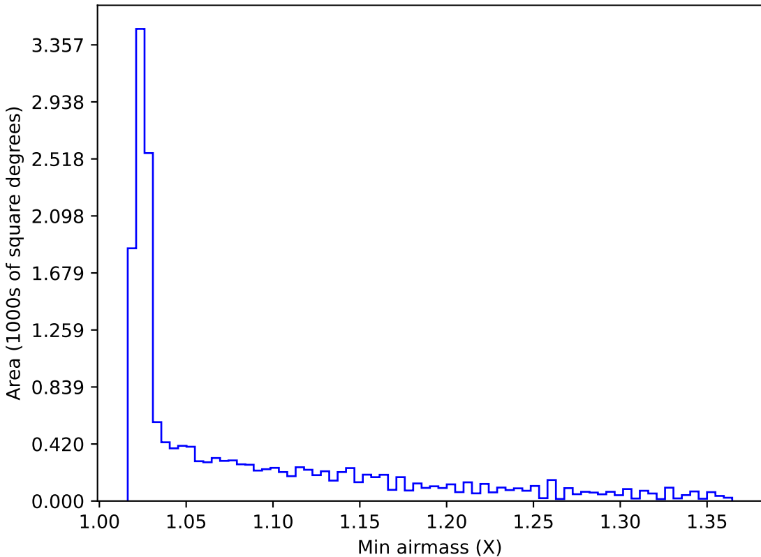
ddf_acor_sf10_lsf40_lsr50_v3.4_10yrs WFD all bands: Min airmass
