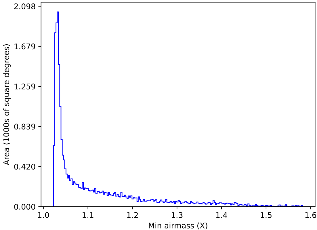
ddf_acor_sf10_lsf40_lsr50_v3.4_10yrs All sky y band: Min airmass
