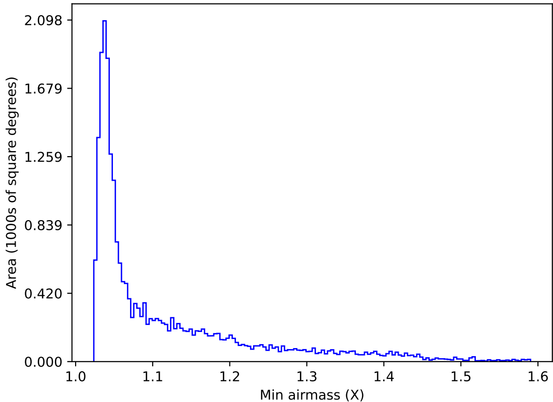
ddf_acor_sf10_lsf40_lsr50_v3.4_10yrs All sky u band: Min airmass
