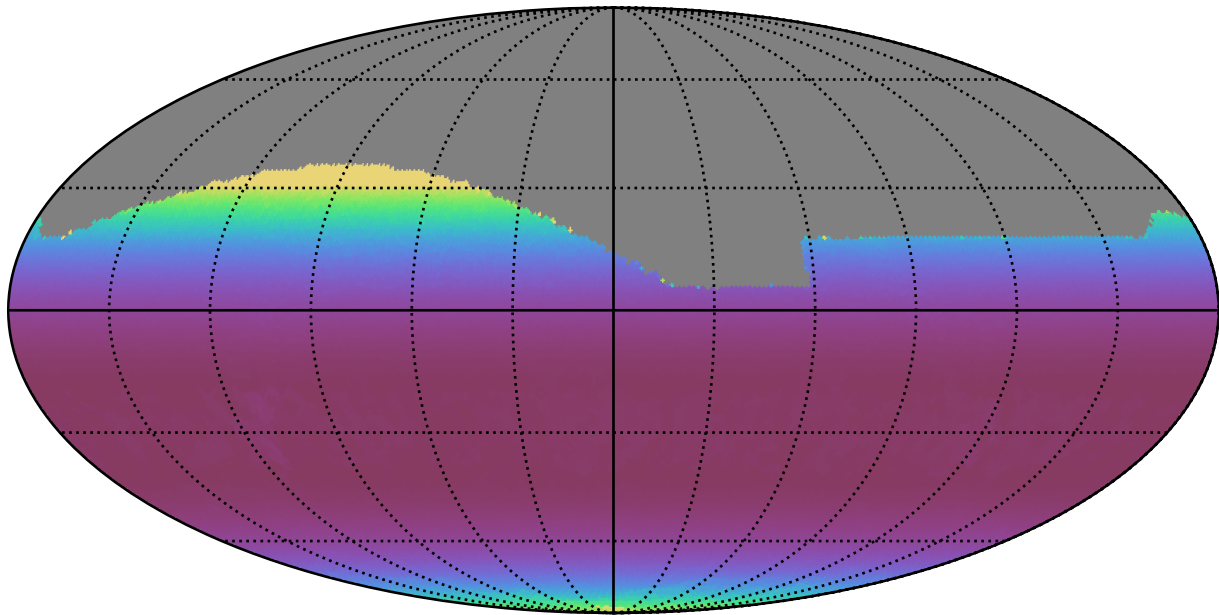
ddf_acor_sf10_lsf40_lsr50_v3.4_10yrs All sky r band: Min airmass
