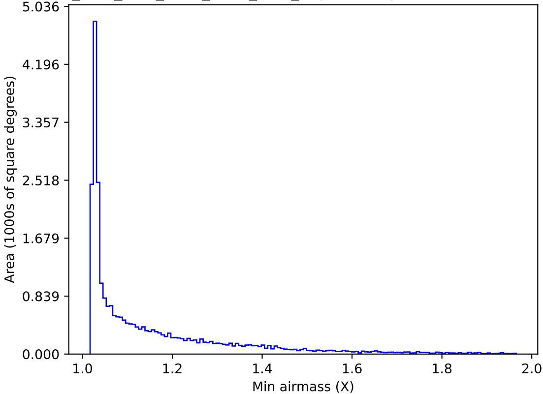
ddf_acor_sf10_lsf40_lsr50_v3.4_10yrs All sky r band: Min airmass
