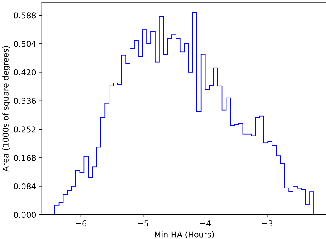
ddf_acor_sf10_lsf40_lsr50_v3.4_10yrs WFD r band: Min HA
