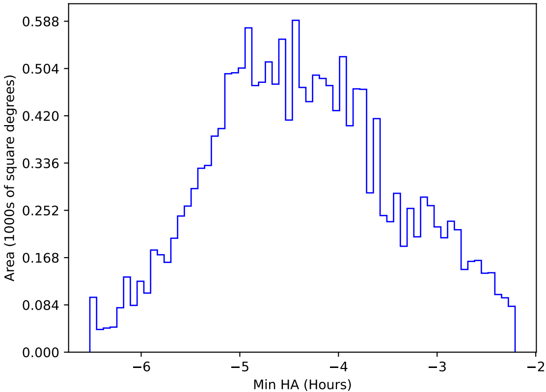
ddf_acor_sf10_lsf40_lsr50_v3.4_10yrs WFD i band: Min HA
