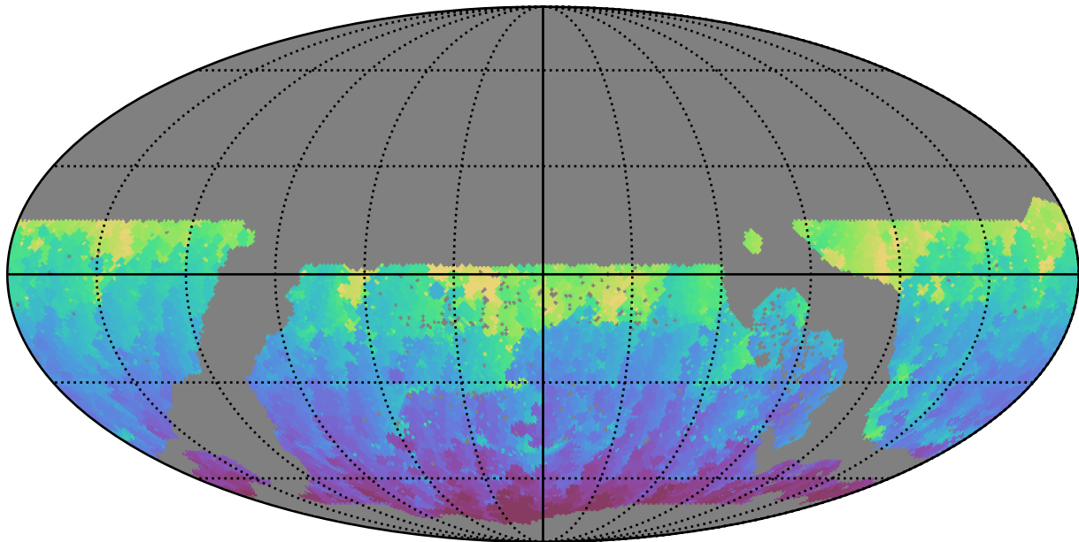
ddf_acor_sf10_lsf40_lsr50_v3.4_10yrs WFD g band: Min HA
