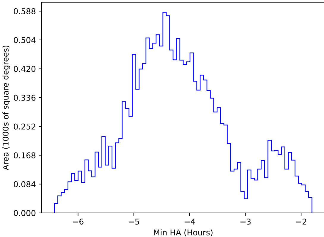
ddf_acor_sf10_lsf40_lsr50_v3.4_10yrs WFD g band: Min HA
