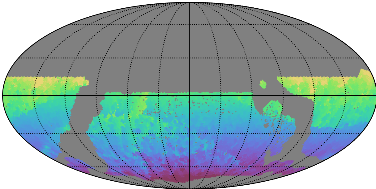
ddf_acor_sf10_lsf40_lsr50_v3.4_10yrs WFD all bands: Min HA
