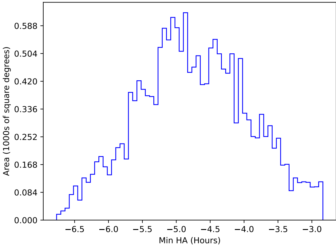
ddf_acor_sf10_ls40_lsr50_v3.4_10yrs WFD all bands: Min HA
