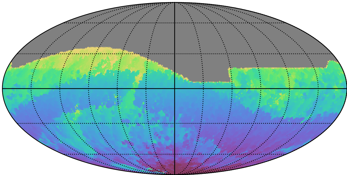
ddf_acor_sf10_lsf40_lsr50_v3.4_10yrs All sky r band: Min HA
