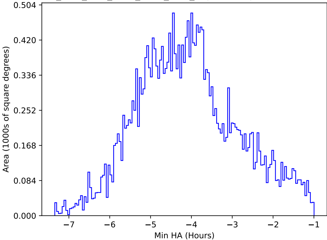
ddf_acor_sf10_ls40_lsr50_v3.4_10yrs All sky i band: Min HA
