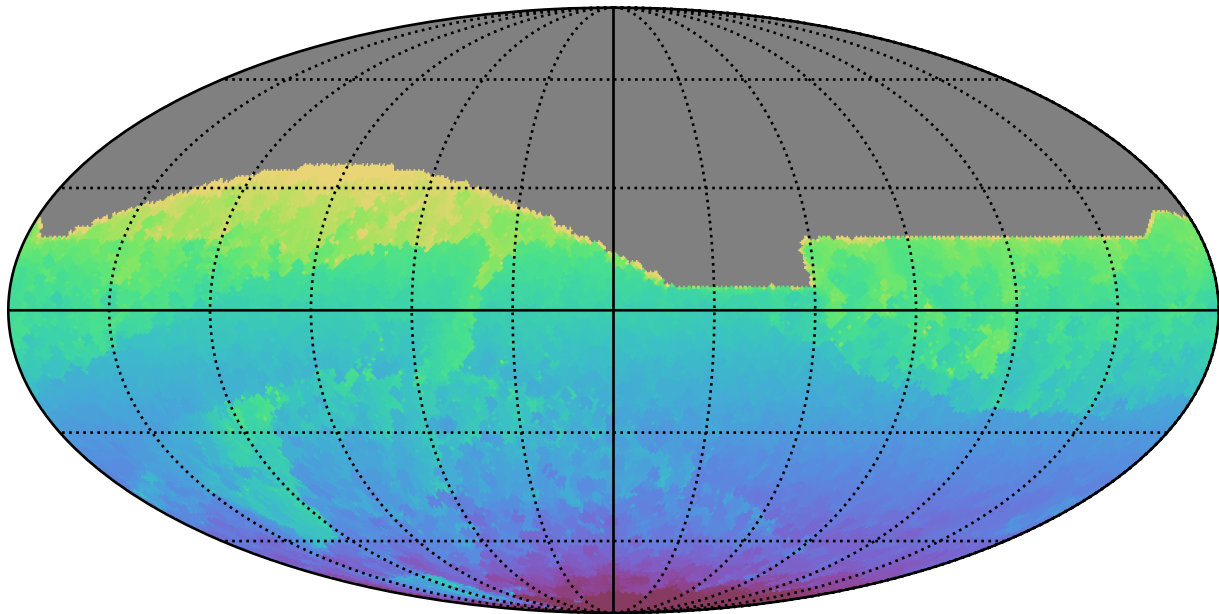
ddf_acor_sf10_lsf40_lsr50_v3.4_10yrs All sky all bands: Min HA
