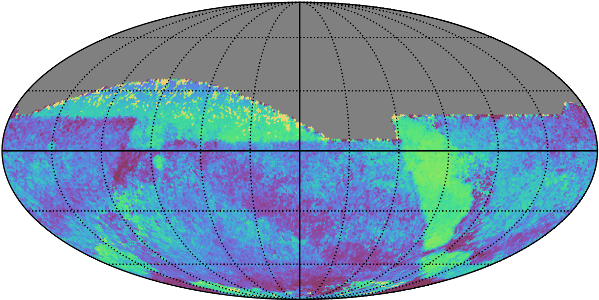
ddf_acor_sf10_lsf40_lsr50_v3.4_10yrs All sky all bands: Median skyBrightness
