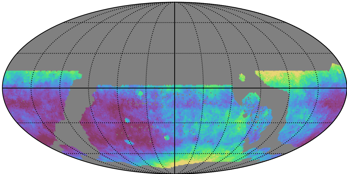
ddf_acor_sf10_lsf40_lsr50_v3.4_10yrs WFD i band: Median seeingEff
