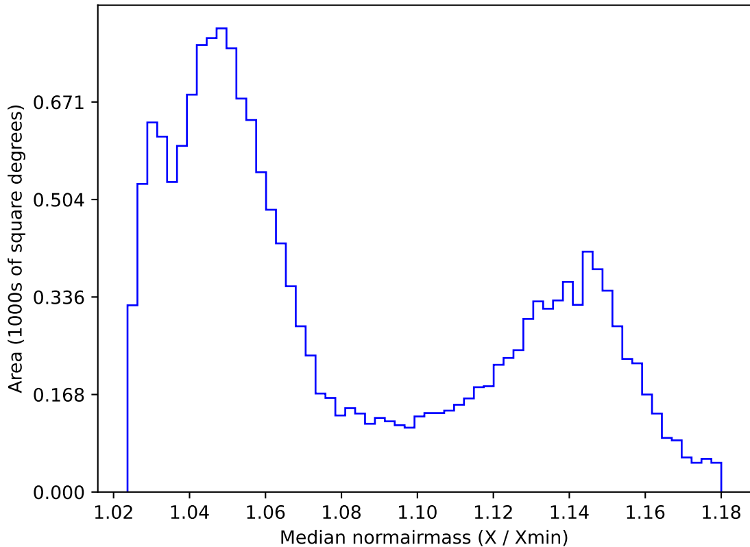
ddf_acor_sf10_lsf40_lsr50_v3.4_10yrs WFD all bands: Median normairmass
