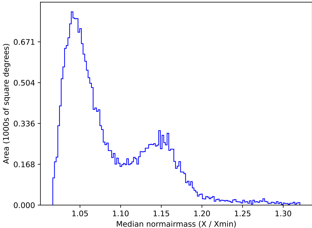
ddf_acor_sf10_lsf40_lsr50_v3.4_10yrs All sky z band: Median normairmass
