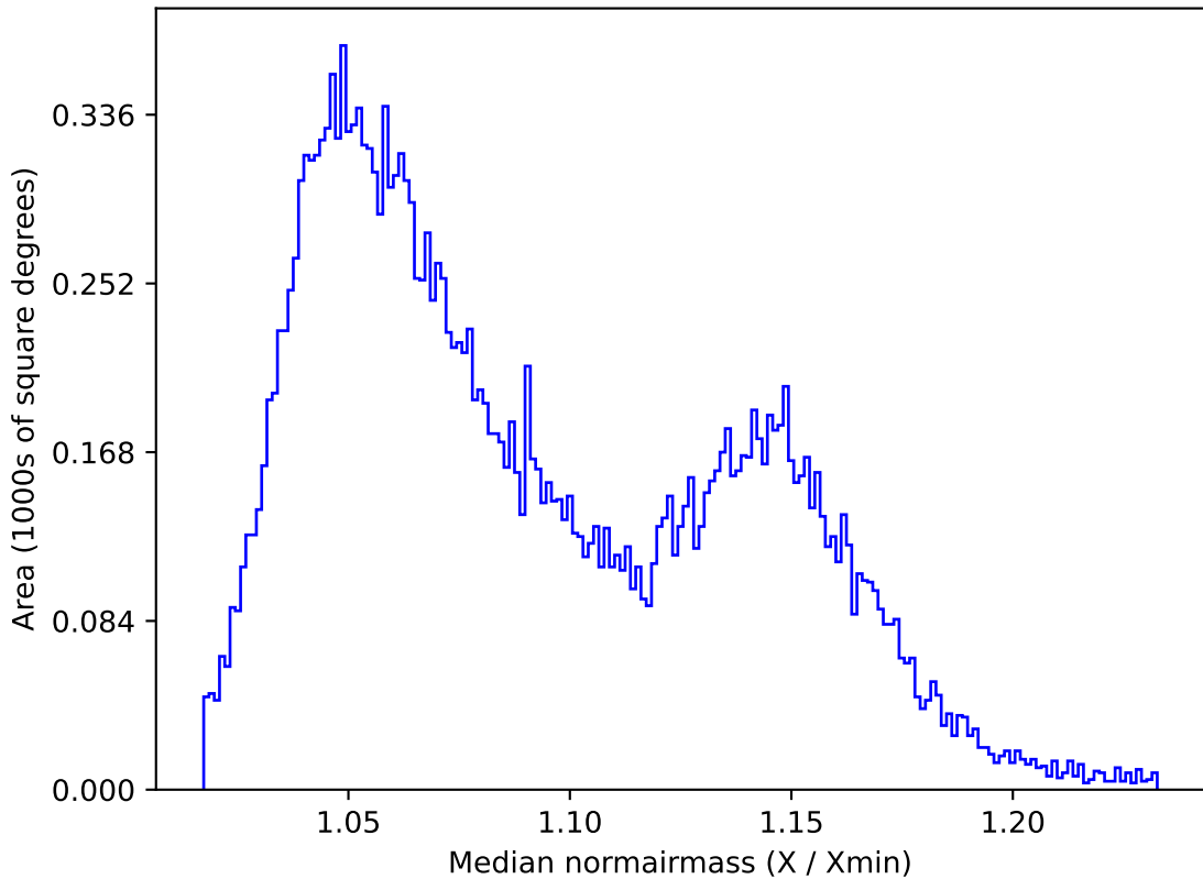
ddf_acor_sf10_lsf40_lsr50_v3.4_10yrs All sky y band: Median normairmass
