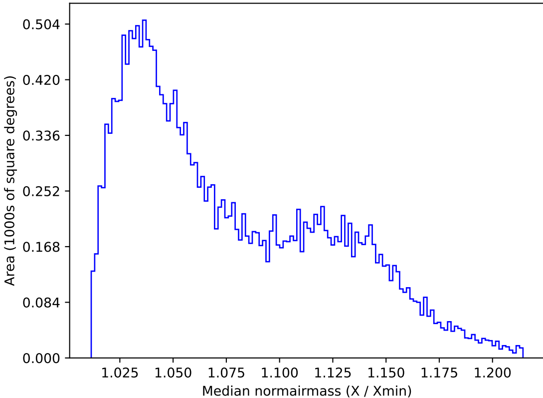
ddf_acor_sf10_ls40_lsr50_v3.4_10yrs All sky u band: Median normairmass
