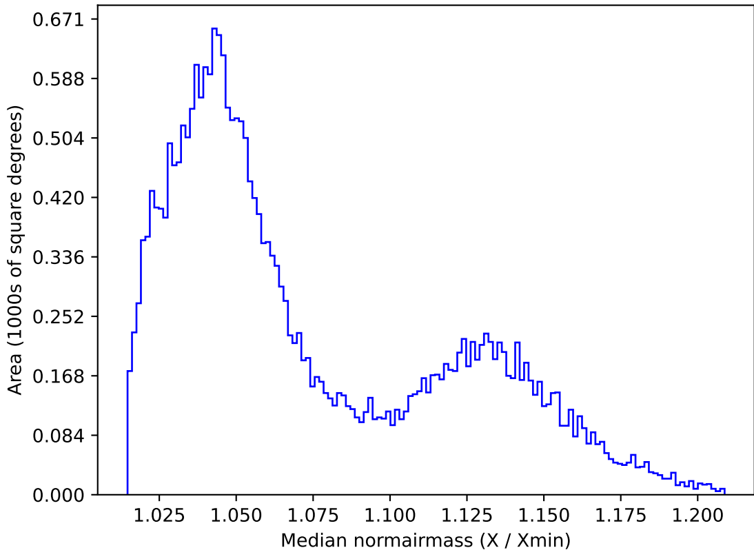
ddf_acor_sf10_lsf40_lsr50_v3.4_10yrs All sky r band: Median normairmass
