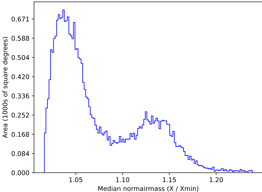
ddf_acor_sf10_lsf40_lsr50_v3.4_10yrs All sky i band: Median normairmass
