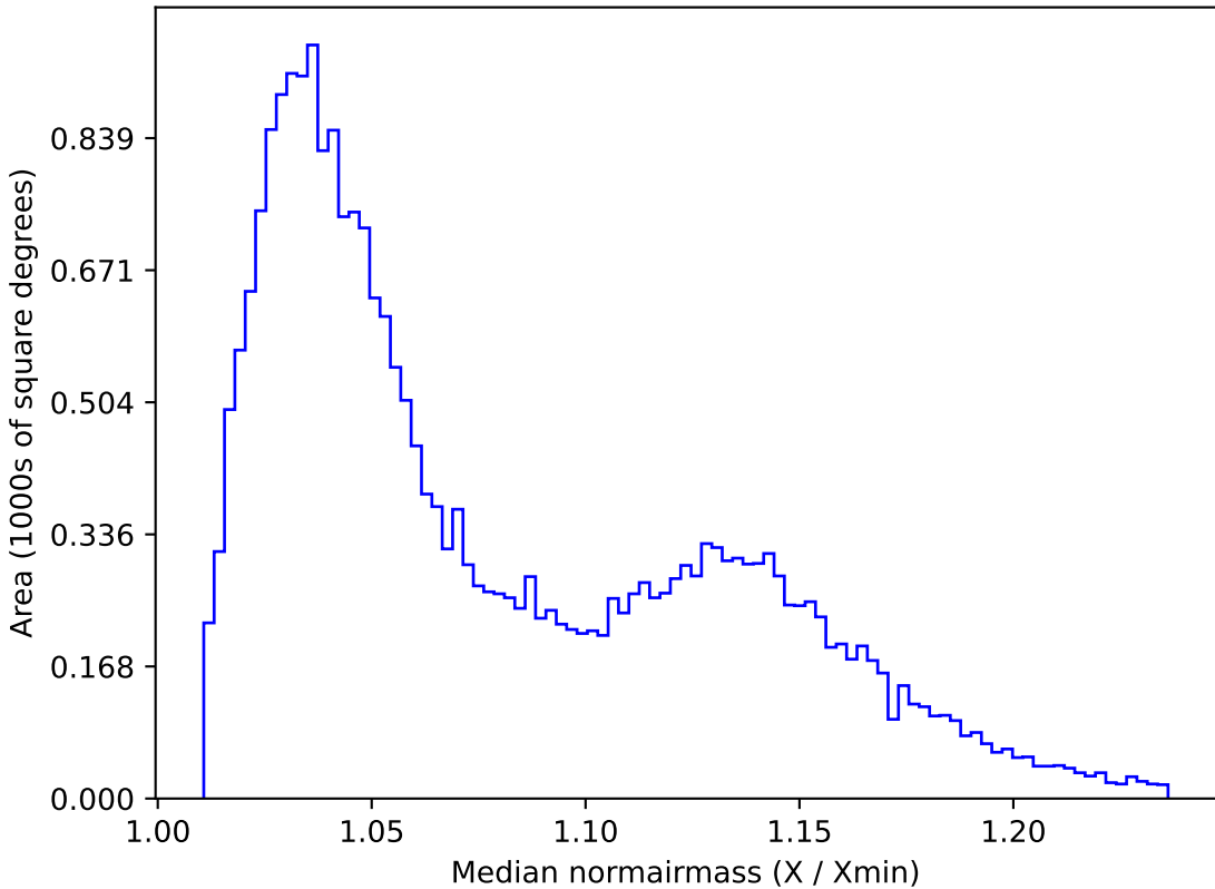
ddf_acor_sf10_lsf40_lsr50_v3.4_10yrs All sky g band: Median normairmass
