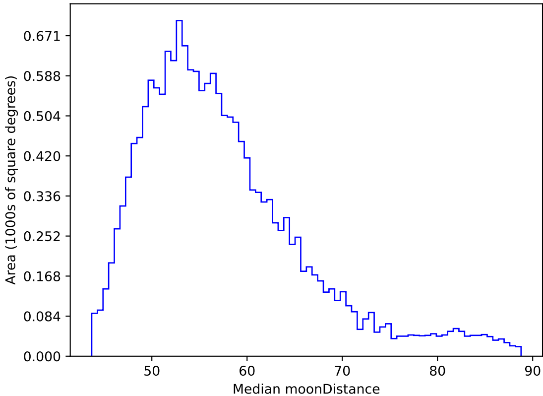
ddf_acor_sf10_lsf40_lsr50_v3.4_10yrs WFD y band: Median moonDistance
