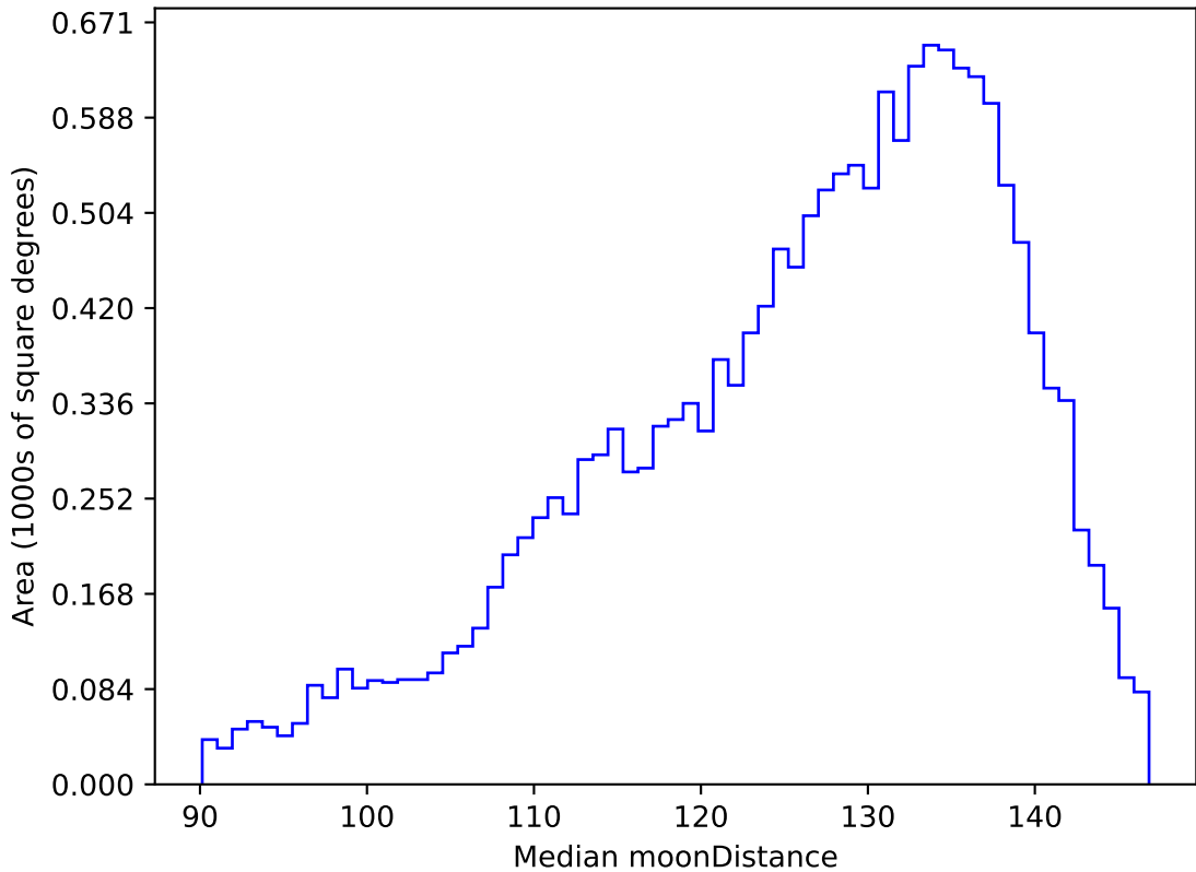
ddf_acor_sf10_lsf40_lsr50_v3.4_10yrs WFD u band: Median moonDistance
